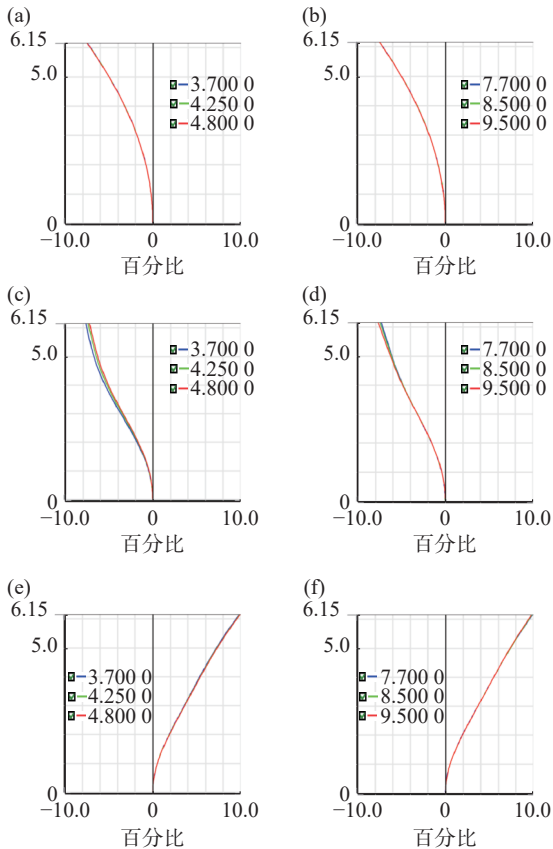
Fig. 5 Distortion curves. (a) MWIR short focus; (b) LWIR short focus; (c) MWIR middle focus; (d) LWIR middle focus; (e) MWIR long focus; (f) LWIR long focus; (g) MWIR super long focus; (h) LWIR super long focus
