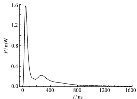
Fig. 5 Waveform of laser pulse power.
