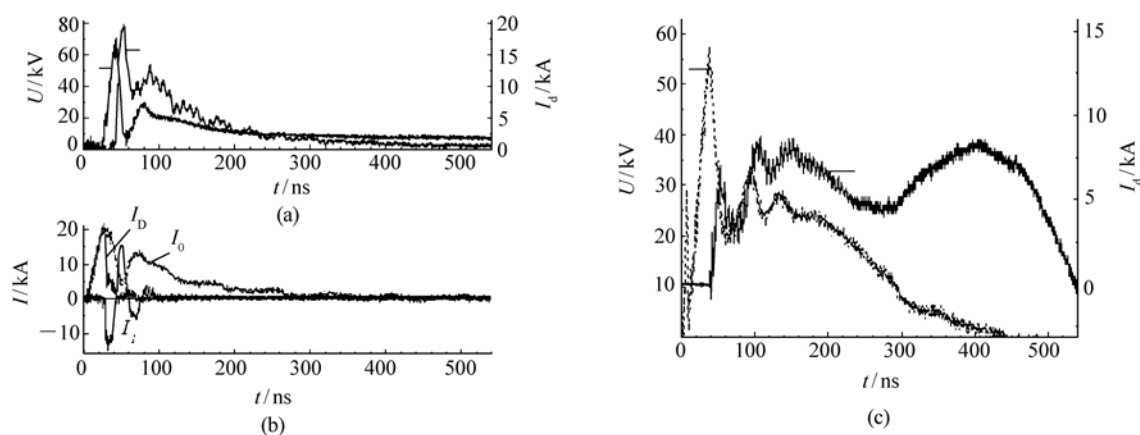
Fig. 4 Oscillograms of voltage pulses across the laser gap ( U ), current in the laser gap ( I_d ), current through the diodes ( I_{DOS} ), and currents in the circuits of the storage ( I_0 ) and peaking ( I_1 ) capacitors. The He:CO 2 :N 2 = 3:1:1 mixture at p \approx 101 kPa was pumped by a generator with an SOS ((a), (b); I = 20 kA, E_L = 5 J) and an LC generator (c). The charging voltage of the storage capacitor is U_0 = 36 kV.
