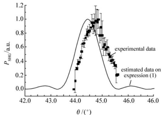
Fig. 9 Dependence of SHG output power on incidence angle \theta for GaSe
